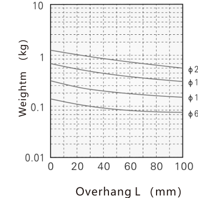
Graph (6) Maximum Speed ≤100 (mm/s) Load eccentricity: 200 (mm)
